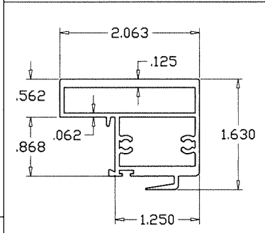
⑥ H.D. MEETING RAIL AT SPRING LATCHES
