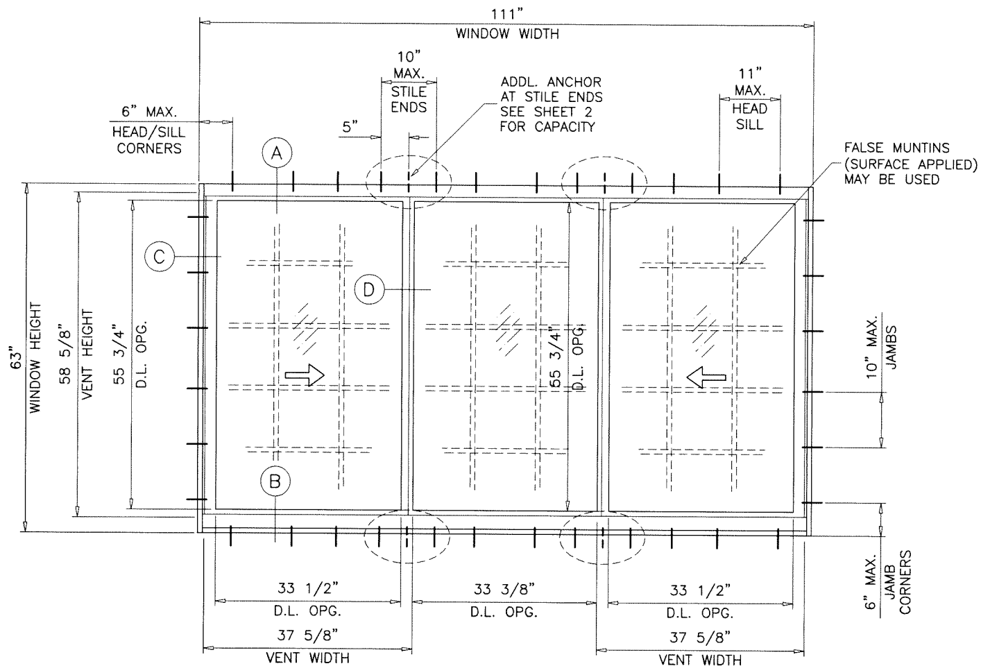
TYPICAL ELEVATION
