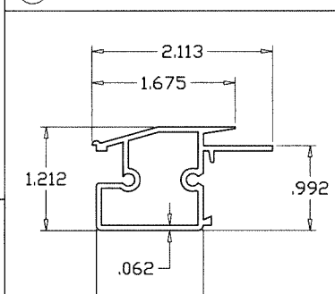
⑥.1 H.D. MEETING RAIL AT SPRING LATCHES
