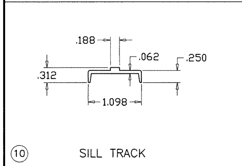
② FRAME SILL
