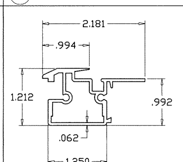
⑥A.1 H.D. MEETING RAIL AT SWEEP LATCHES
